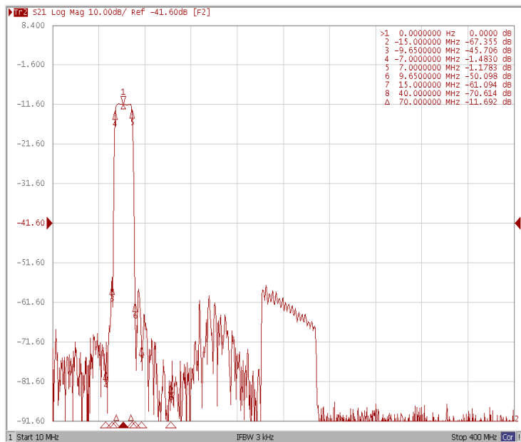
Wide Attenuation
