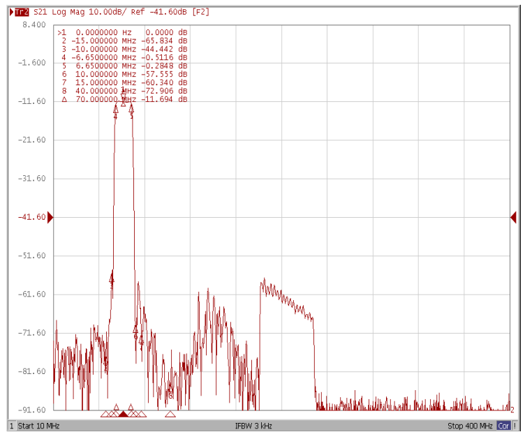
Wide Attenuation
