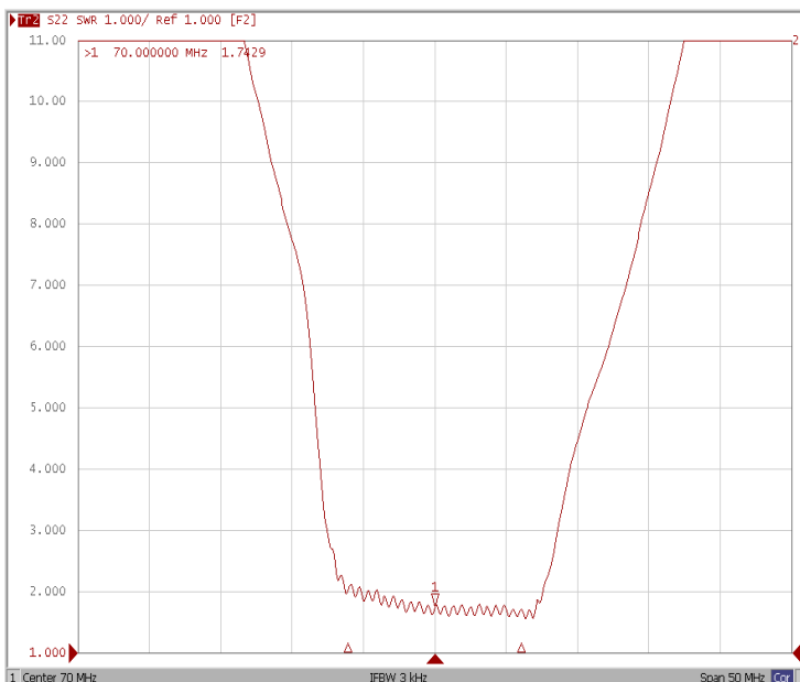
VSWR S22
