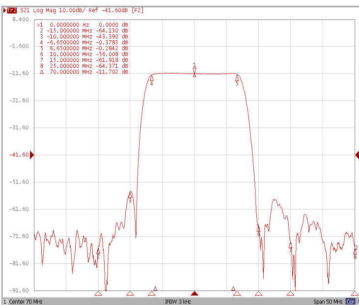
Relative Attenuation
