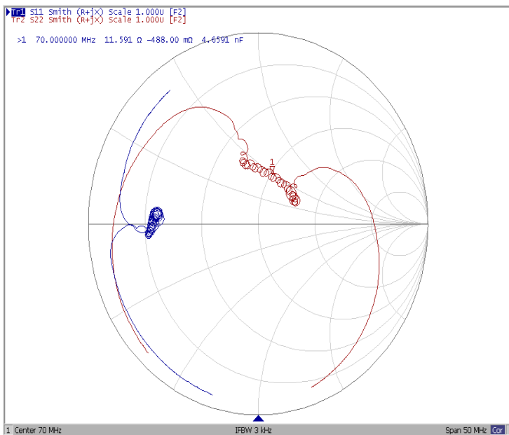
SMITH
