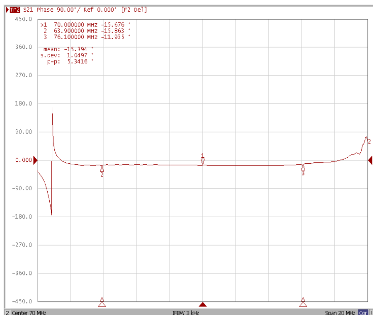
Phase Linearity Fo±6.1MHz
