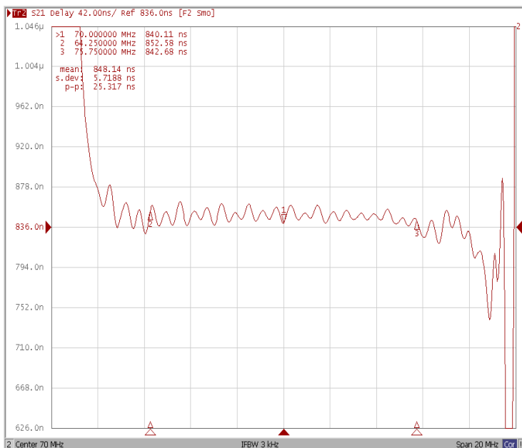
Group Delay Variation Fo±5.75MHz
