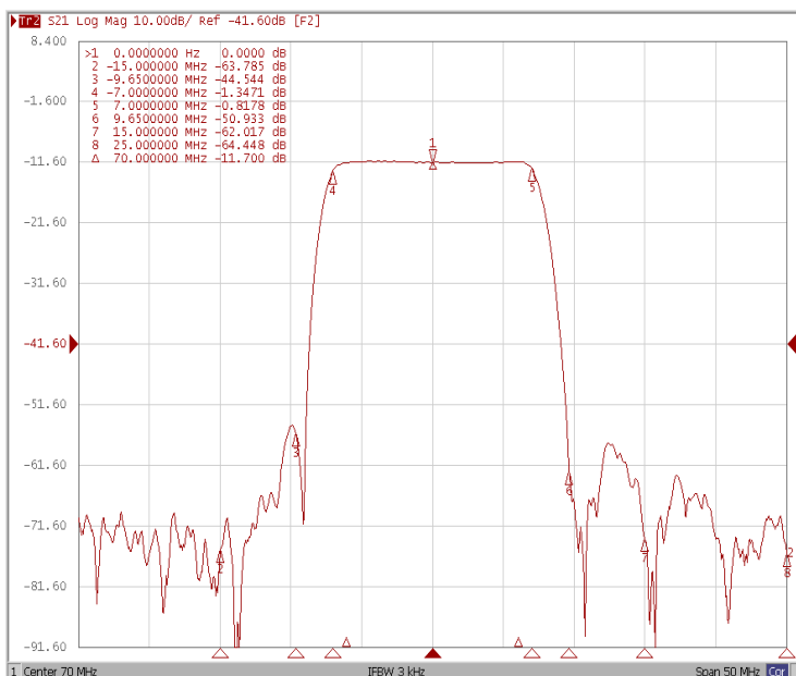
Relative Attenuation
